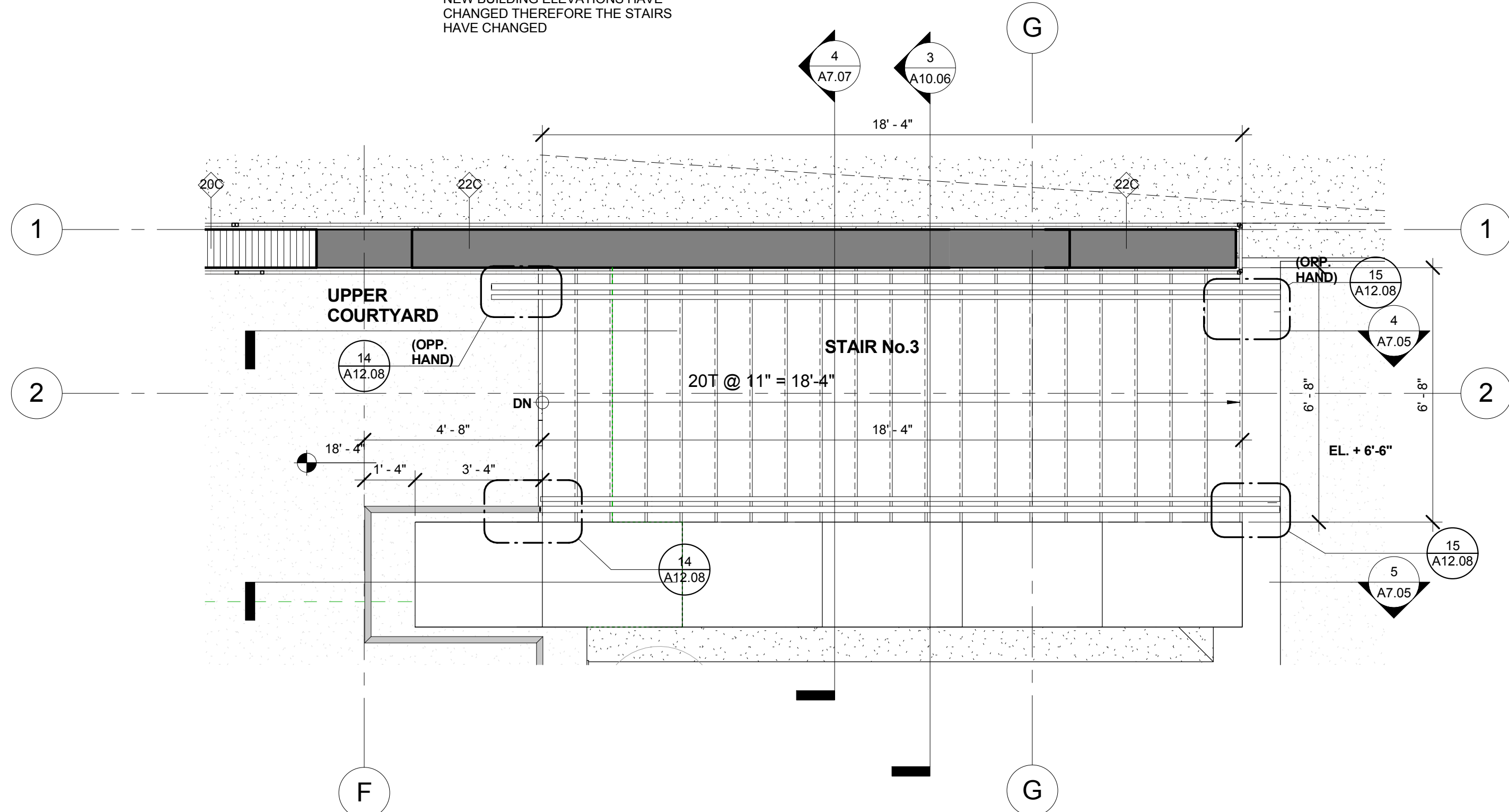
3 STAIR 03 - LEVEL 200
