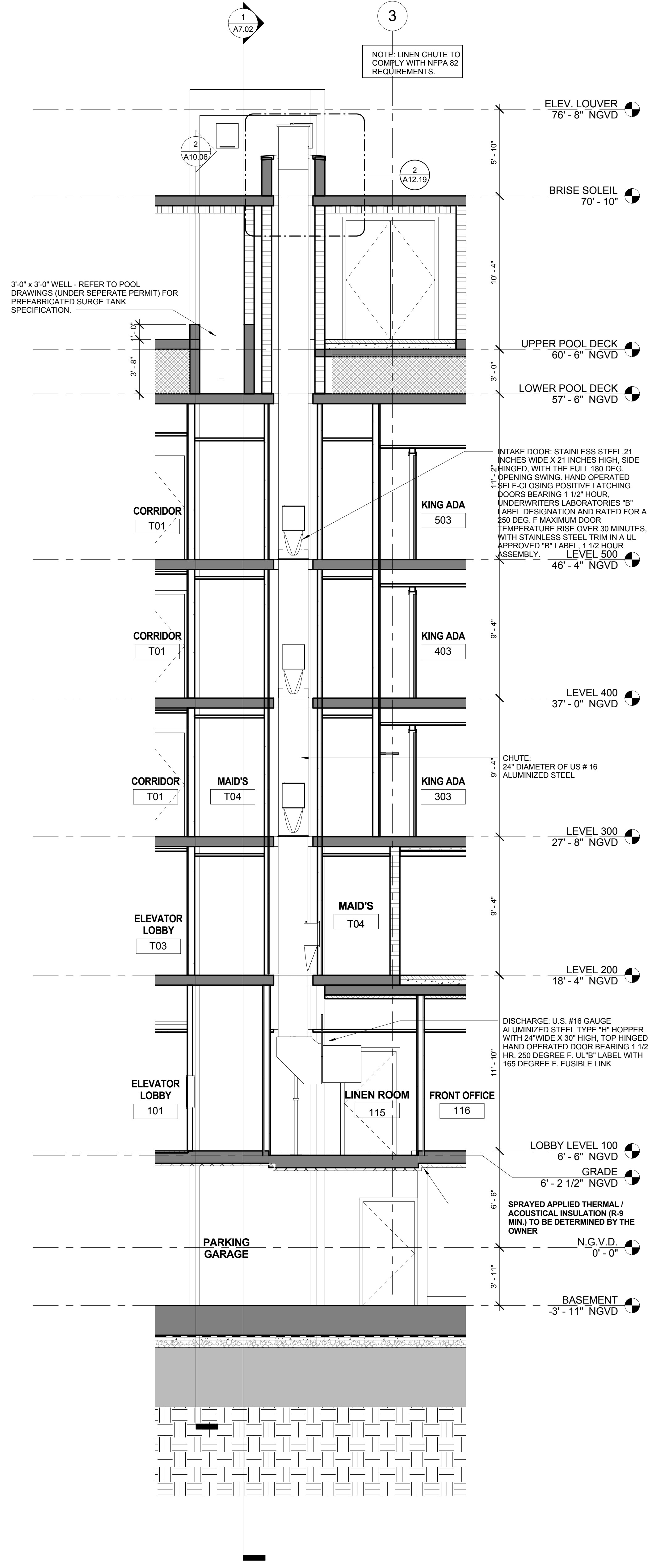
2 A7.02 SECTION-LINEN CHUTE 1/4" = 1'-0"
