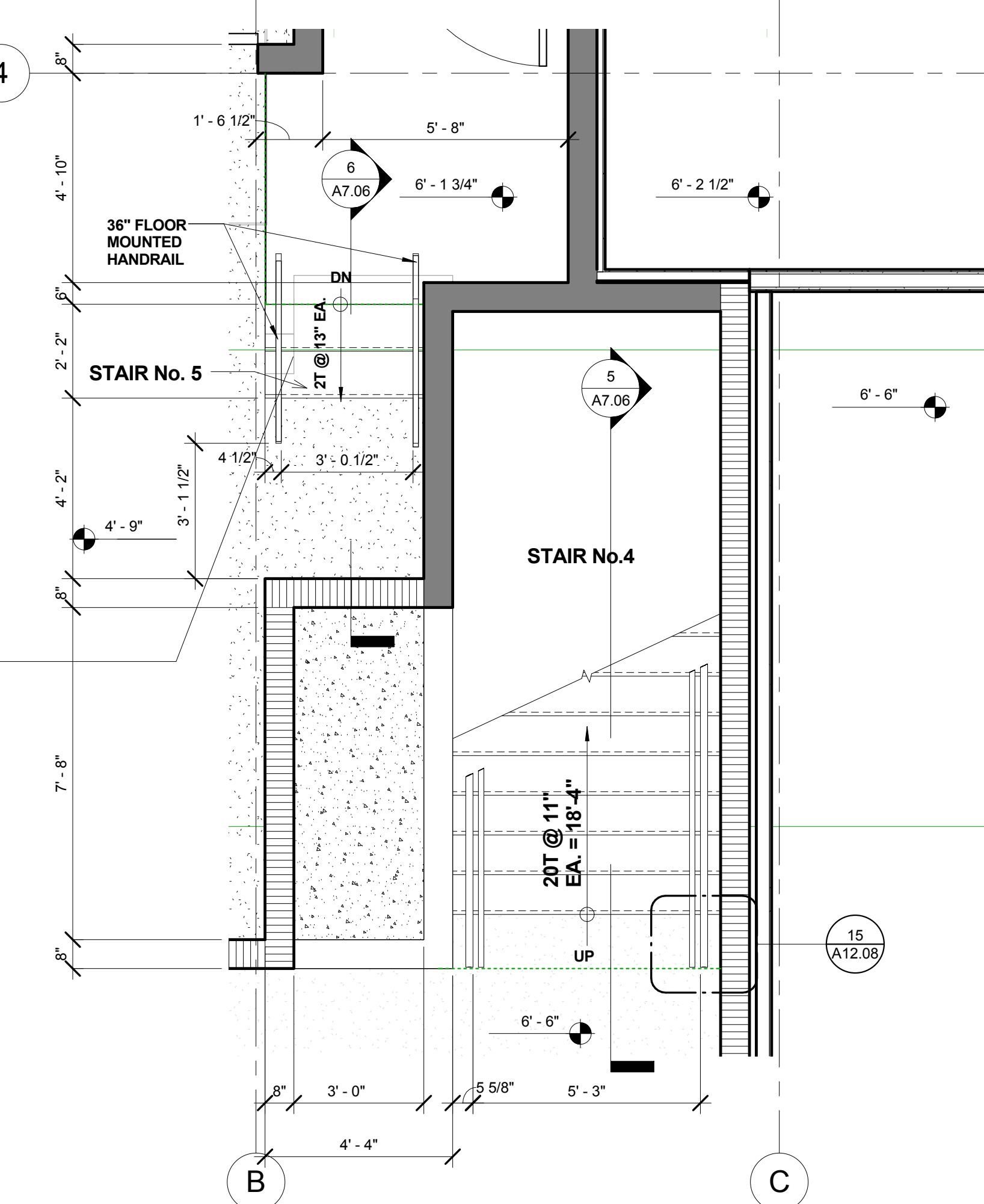
STAIR 04 AND 05 - LEVEL 100
