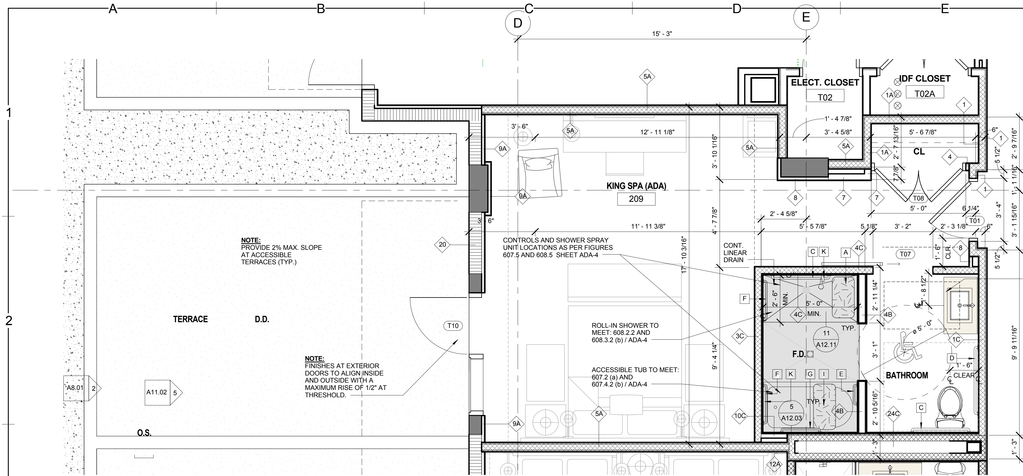
1 KING SPA - B, ADA WITH ROLL-IN SHOWER A5.04 3/8" = 1'-0"
