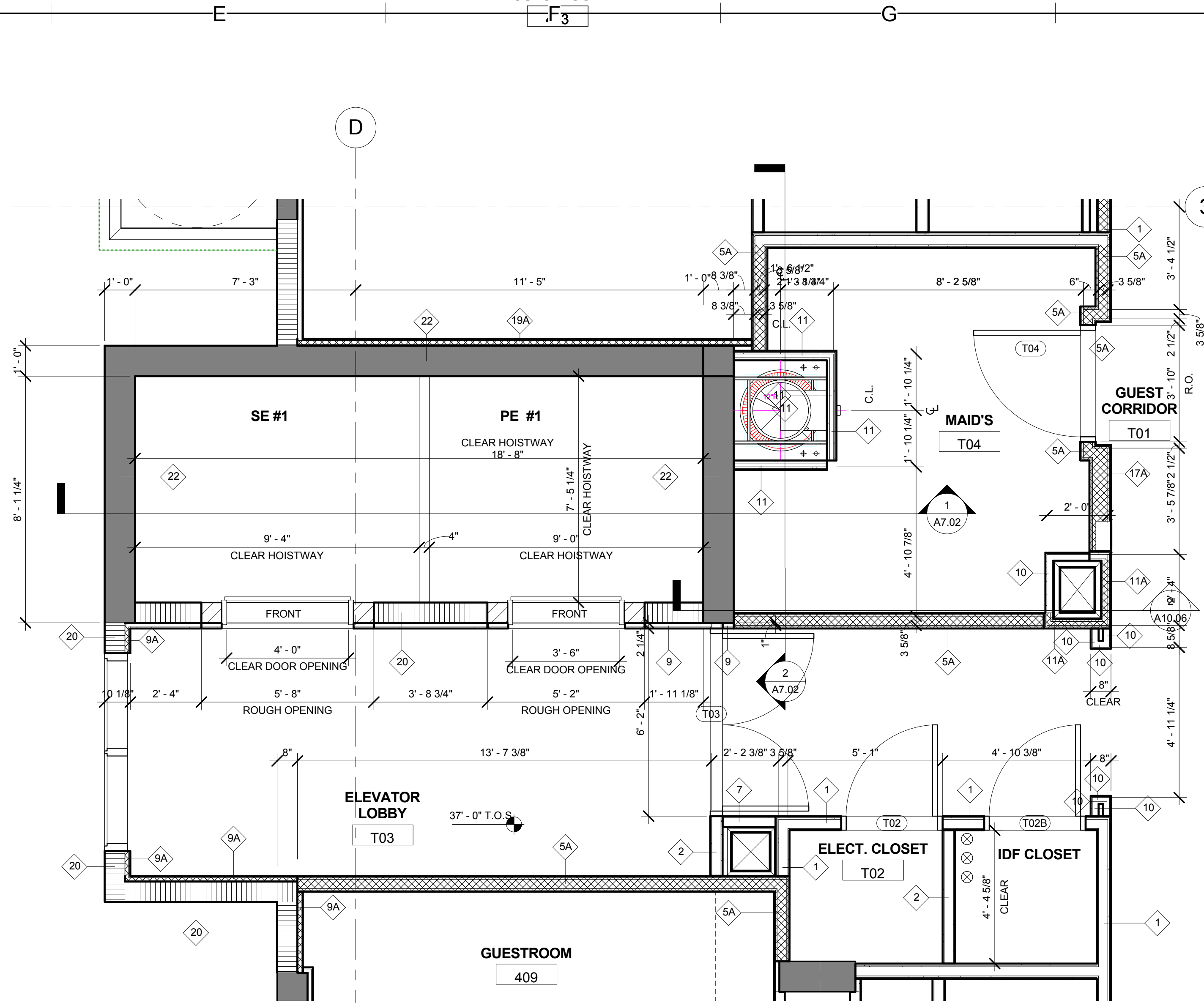
2 ELEVATOR CORE - LEVELS 400 A7.01 3/8" = 1'-0"
