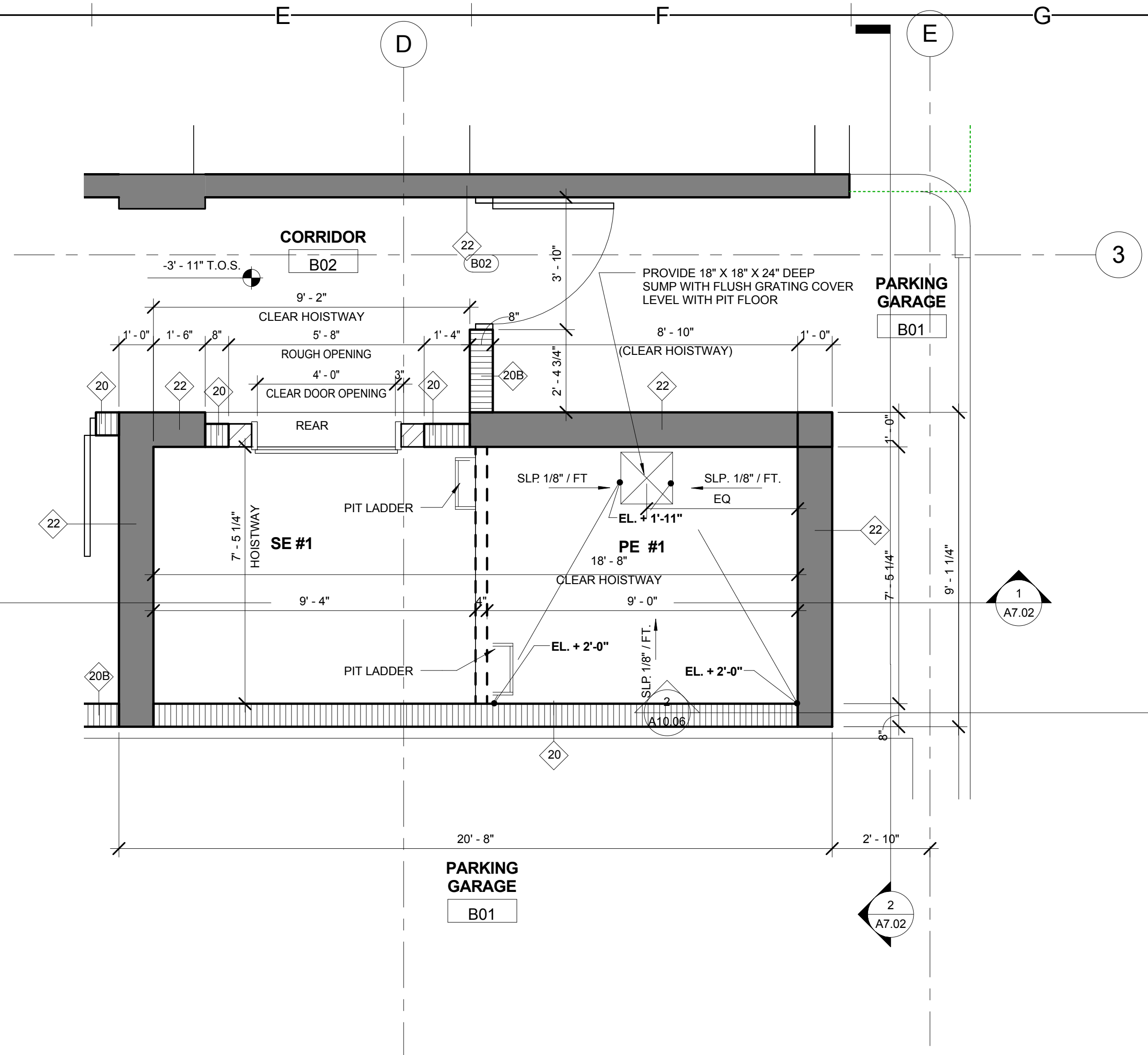
2 A7.00 ELEVATOR CORE - BASEMENT 3/8" = 1'-0"
