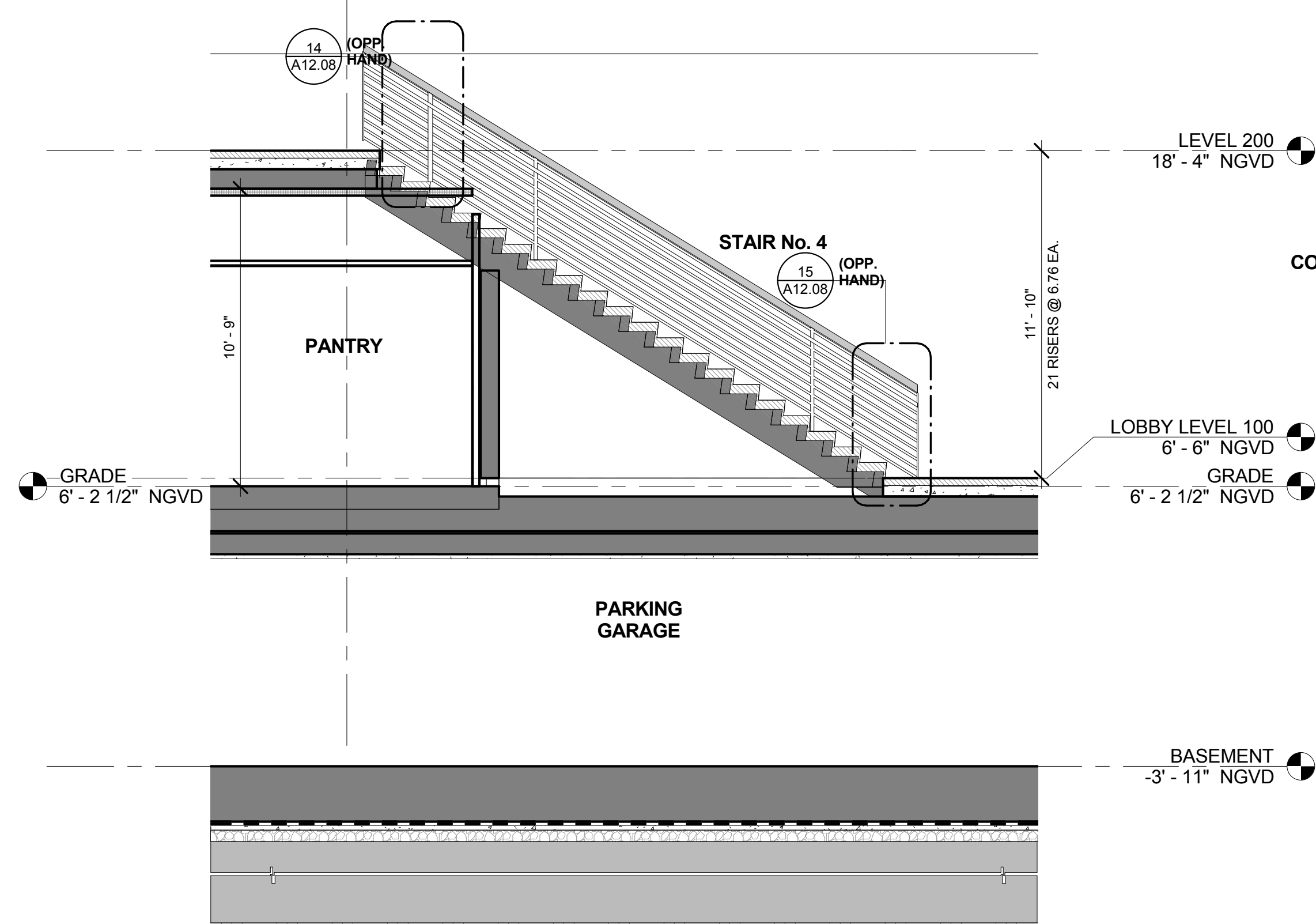
SECTION - STAIR 04
