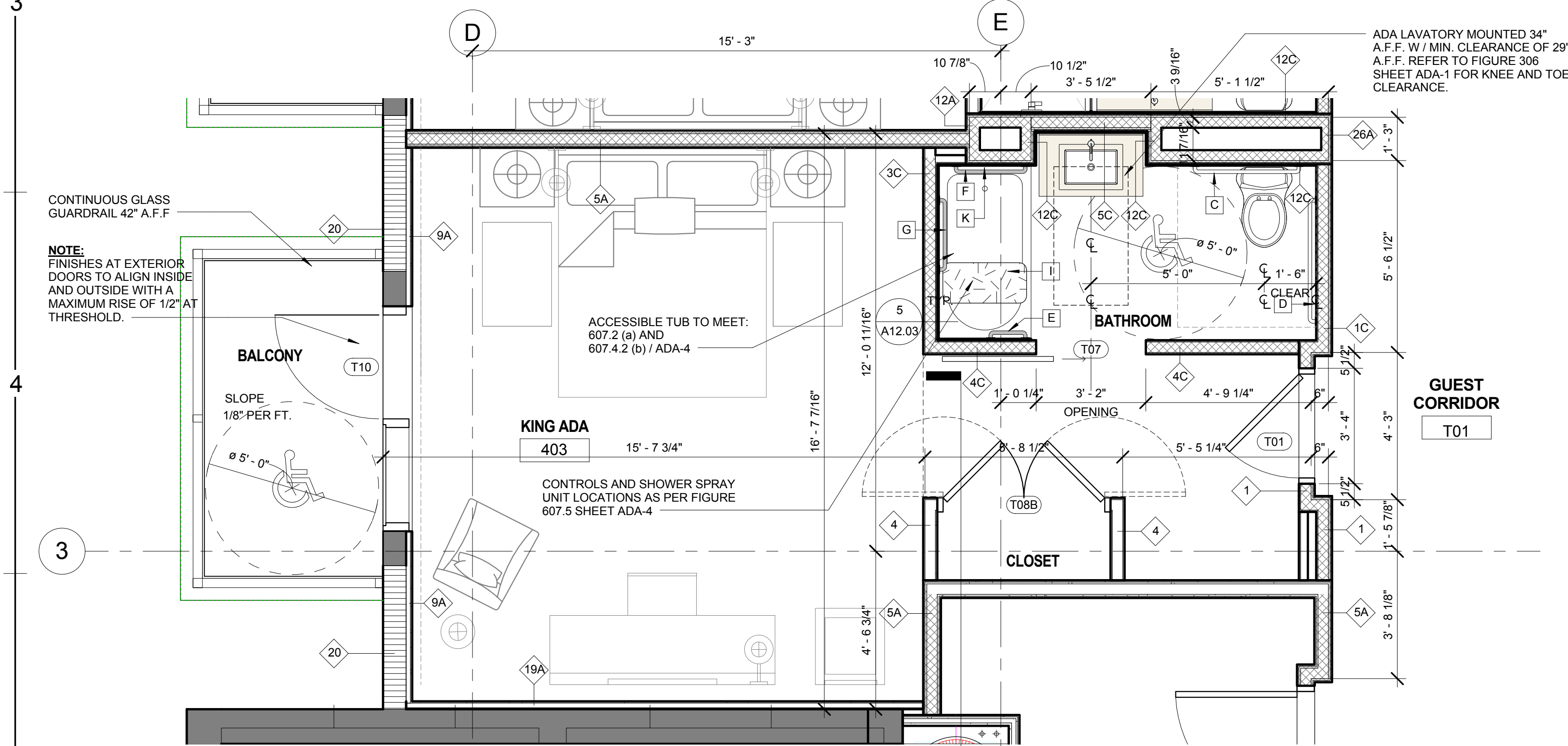
2 KING - ADA WITH TUB A5.04 3/8" = 1'-0"
