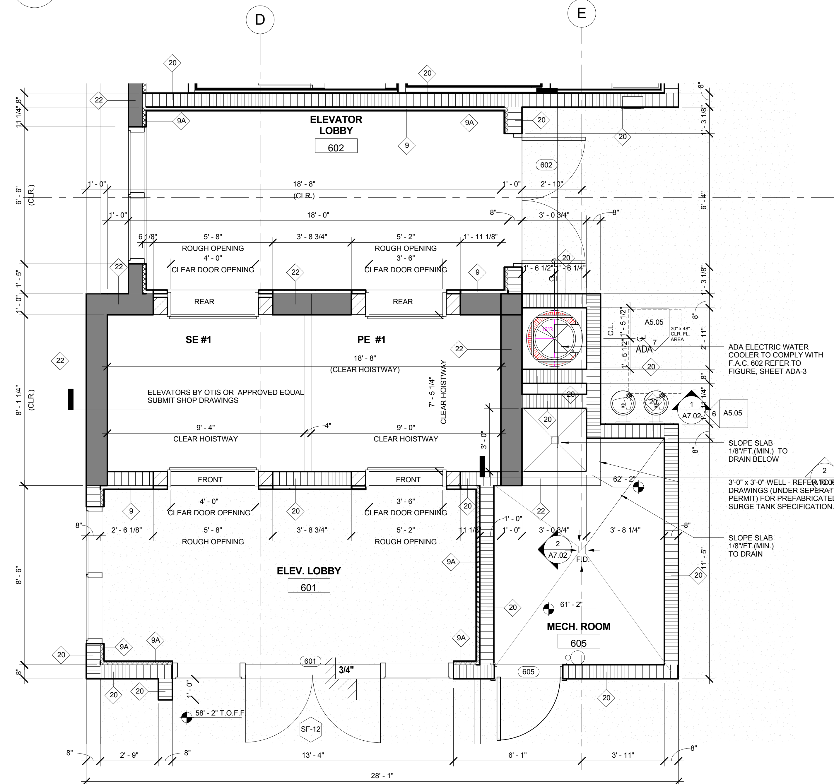
1 ELEVATOR CORE - LEVEL 300 & 500 A7.01 3/8" = 1'-0"
