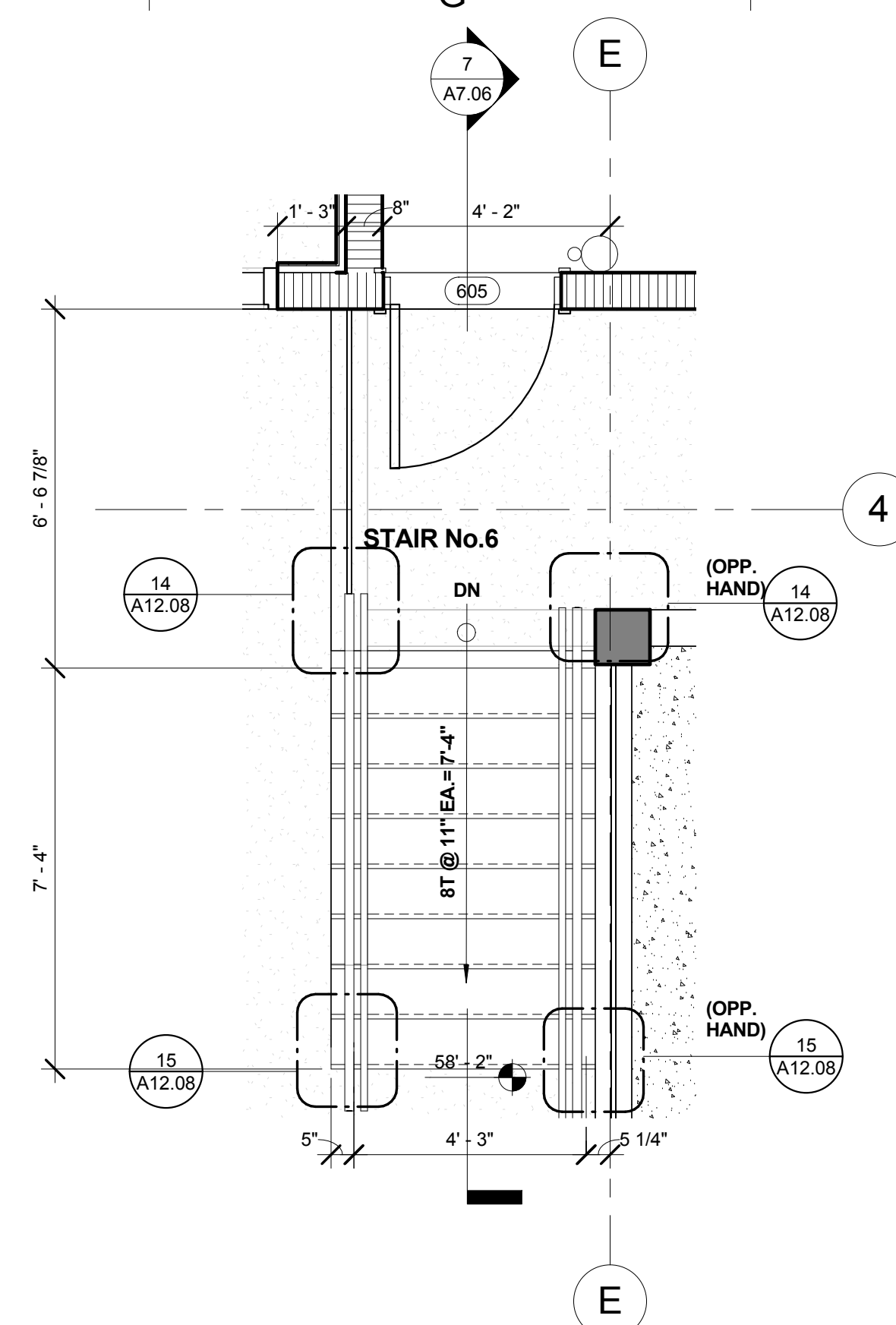
STAIR 06 - LEVEL POOL DECK
