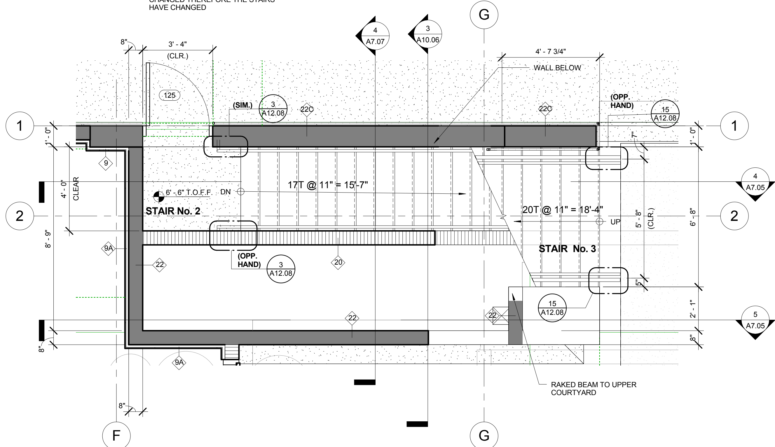
2 STAIR 02 AND 03 - LEVEL 100
