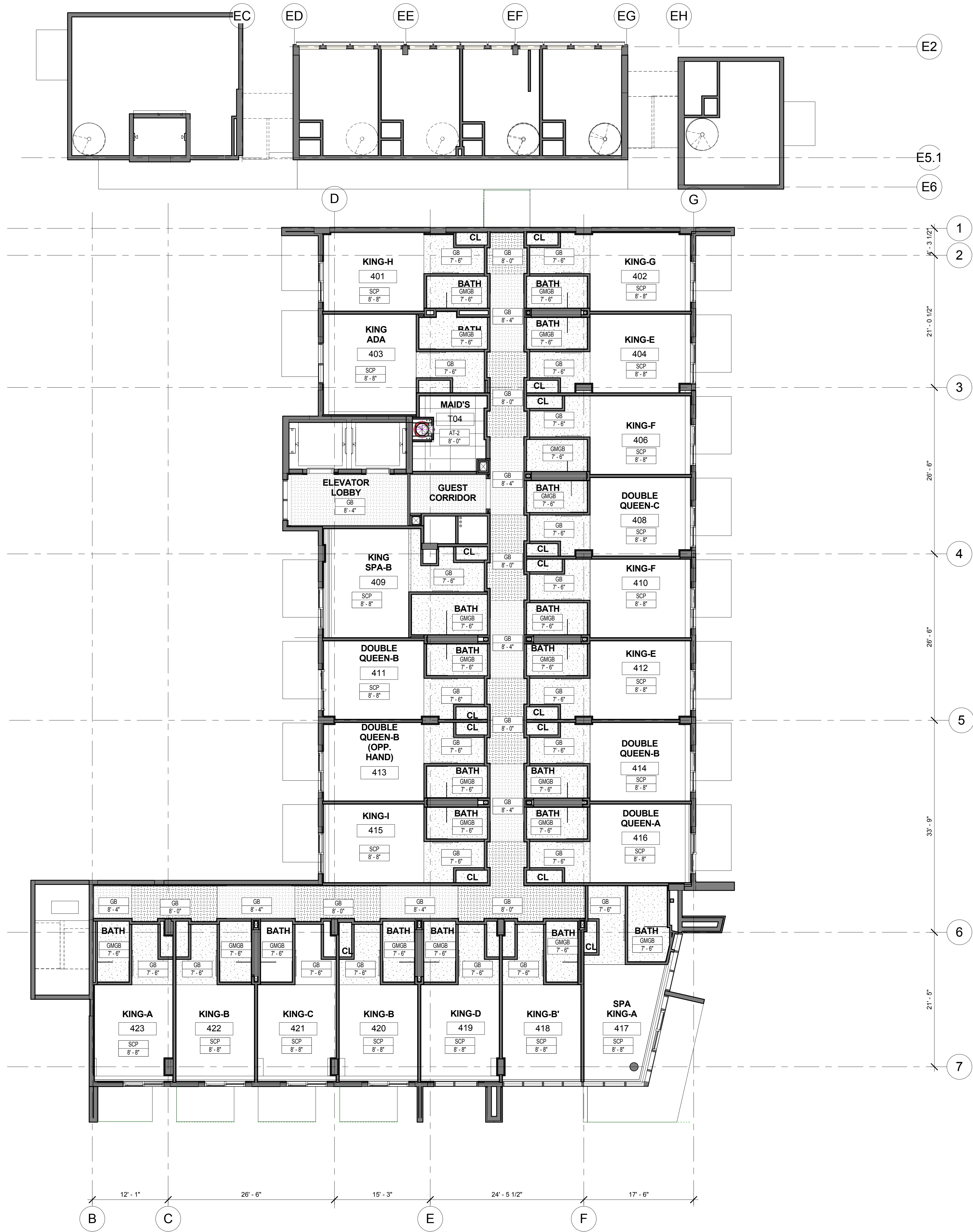
1 A6.04 LEVEL 400 REFLECTED CEILING PLAN 1/8" = 1'-0"
