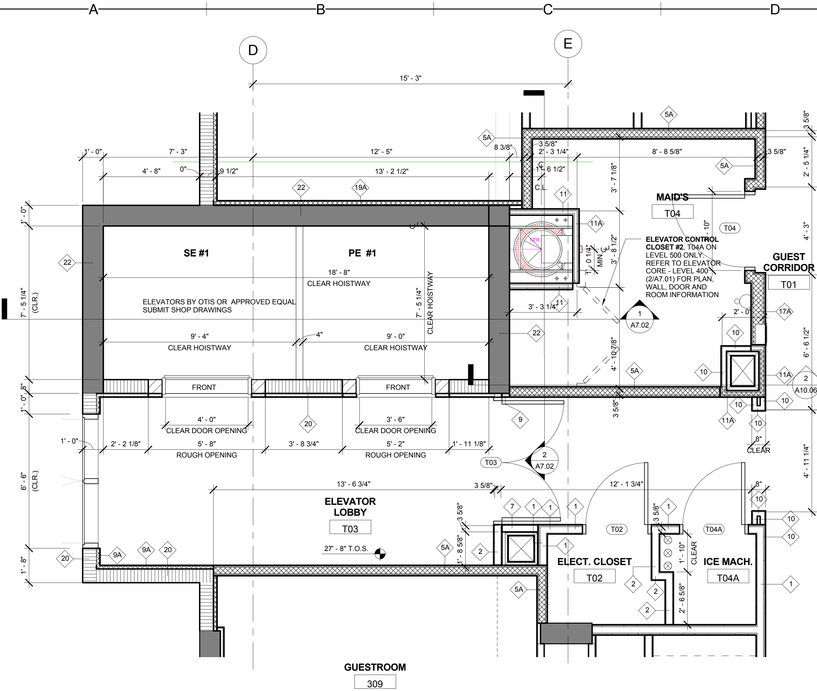
1 ELEVATOR CORE - LEVEL 300 & 500 A7.01 3/8" = 1'-0"
