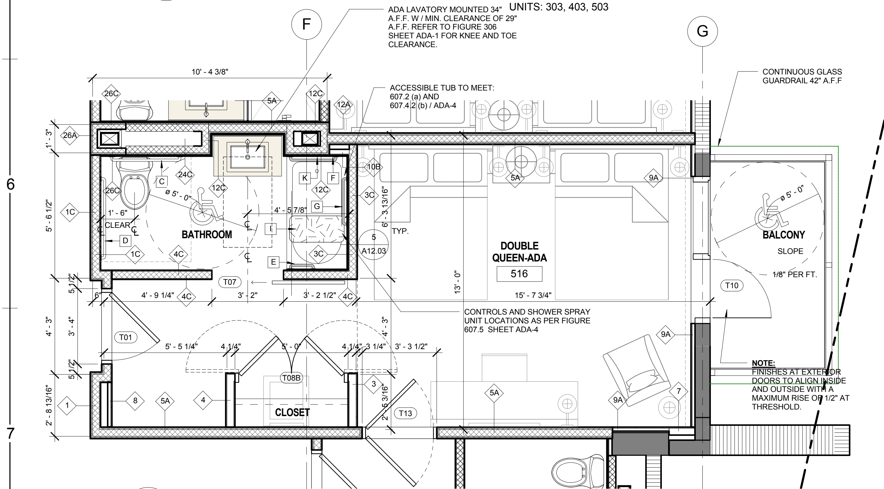
3 DOUBLE QUEEN - ADA WITH TUB A5.04 3/8" = 1'-0"
