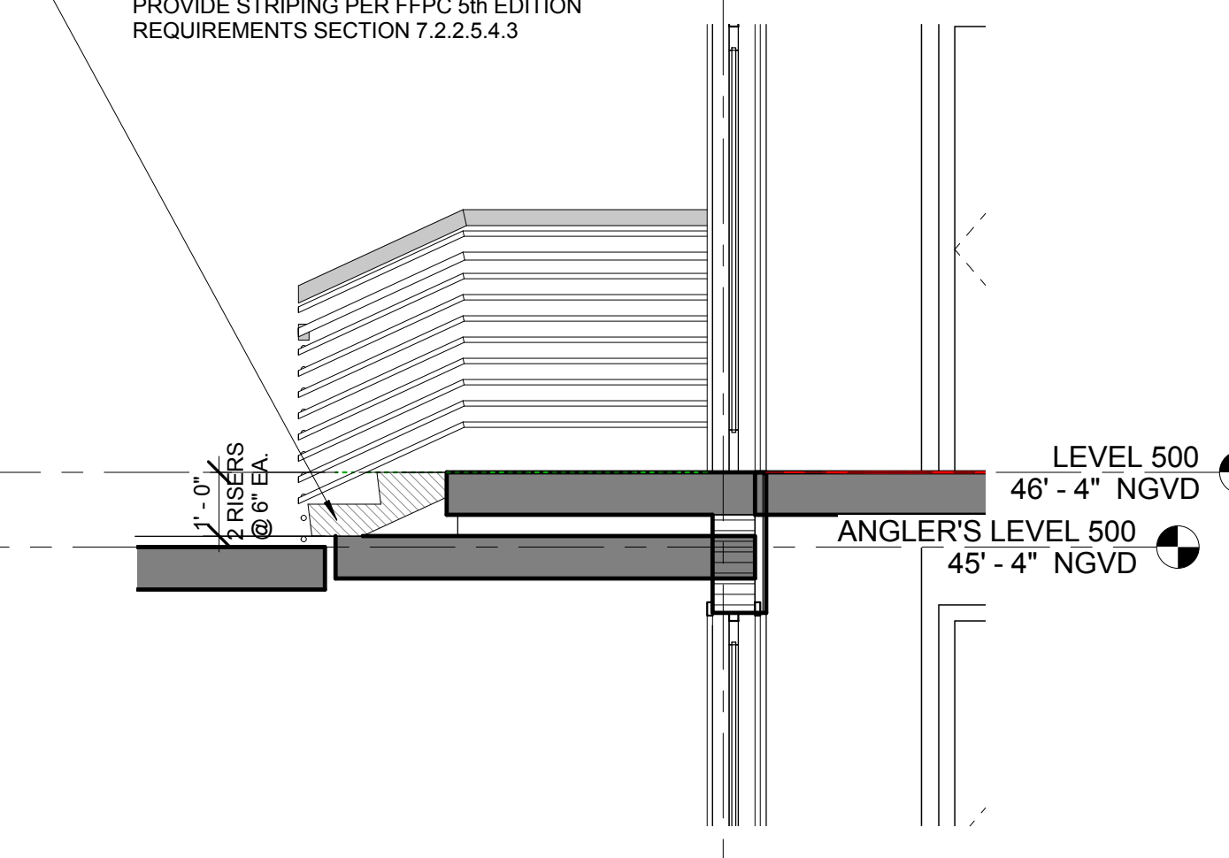
STAIR 11-SECTION
