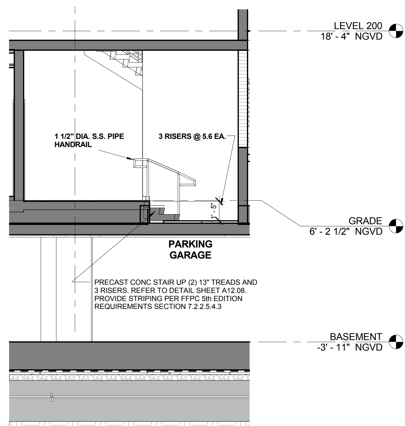
SECTION - STAIR 05
