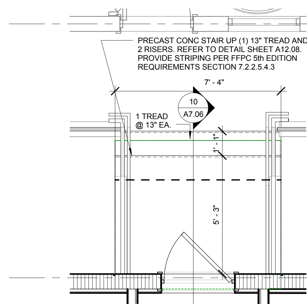
STAIR 11-LEVEL 300,400 AND 500
