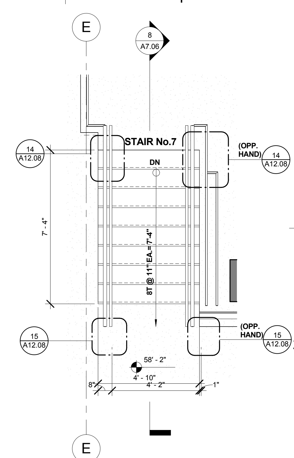
STAIR 07 - LEVEL POOL DECK
