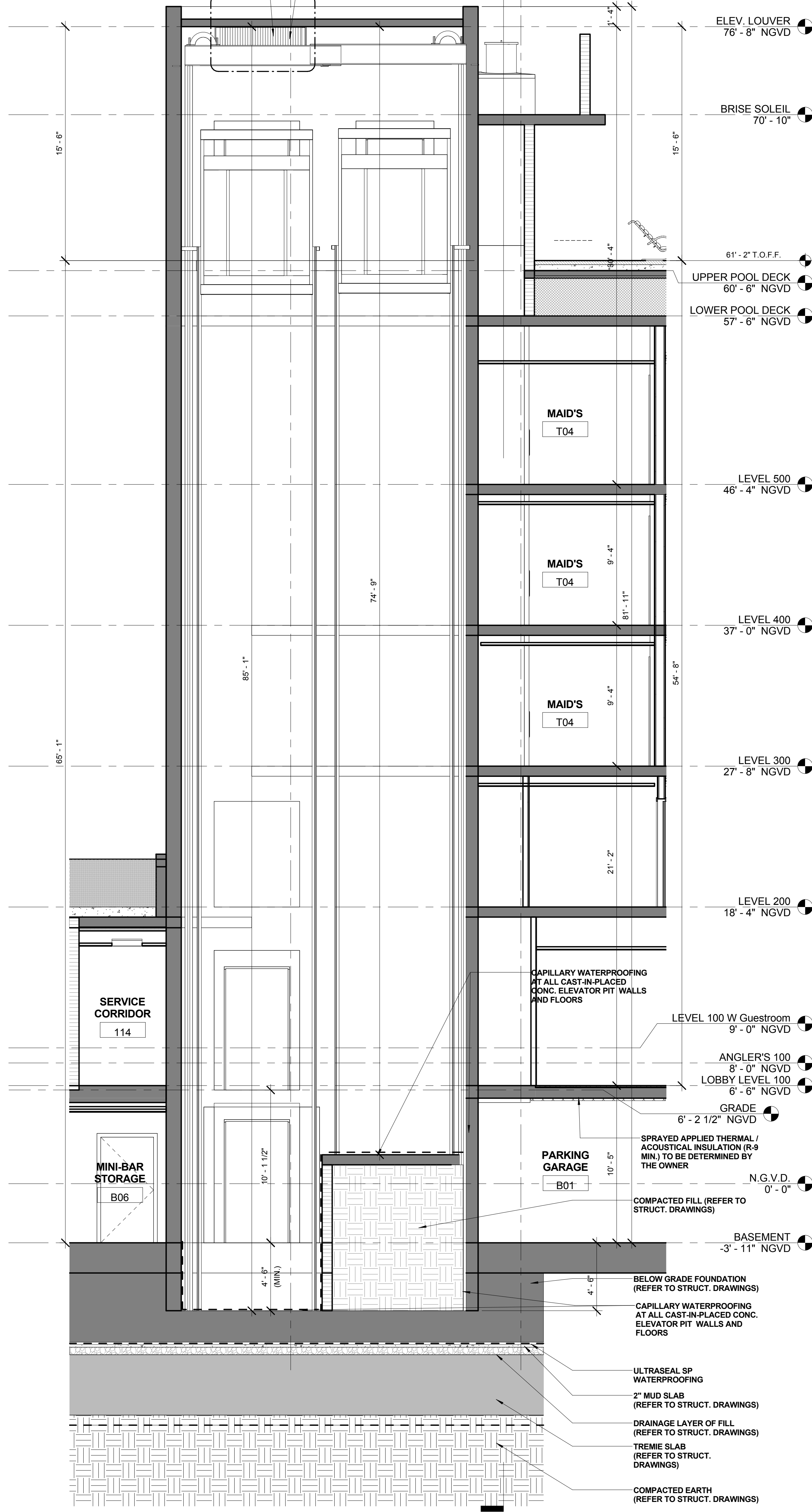
1 A7.02 SECTION - ELEVATOR CORE 1/4" = 1'-0"
