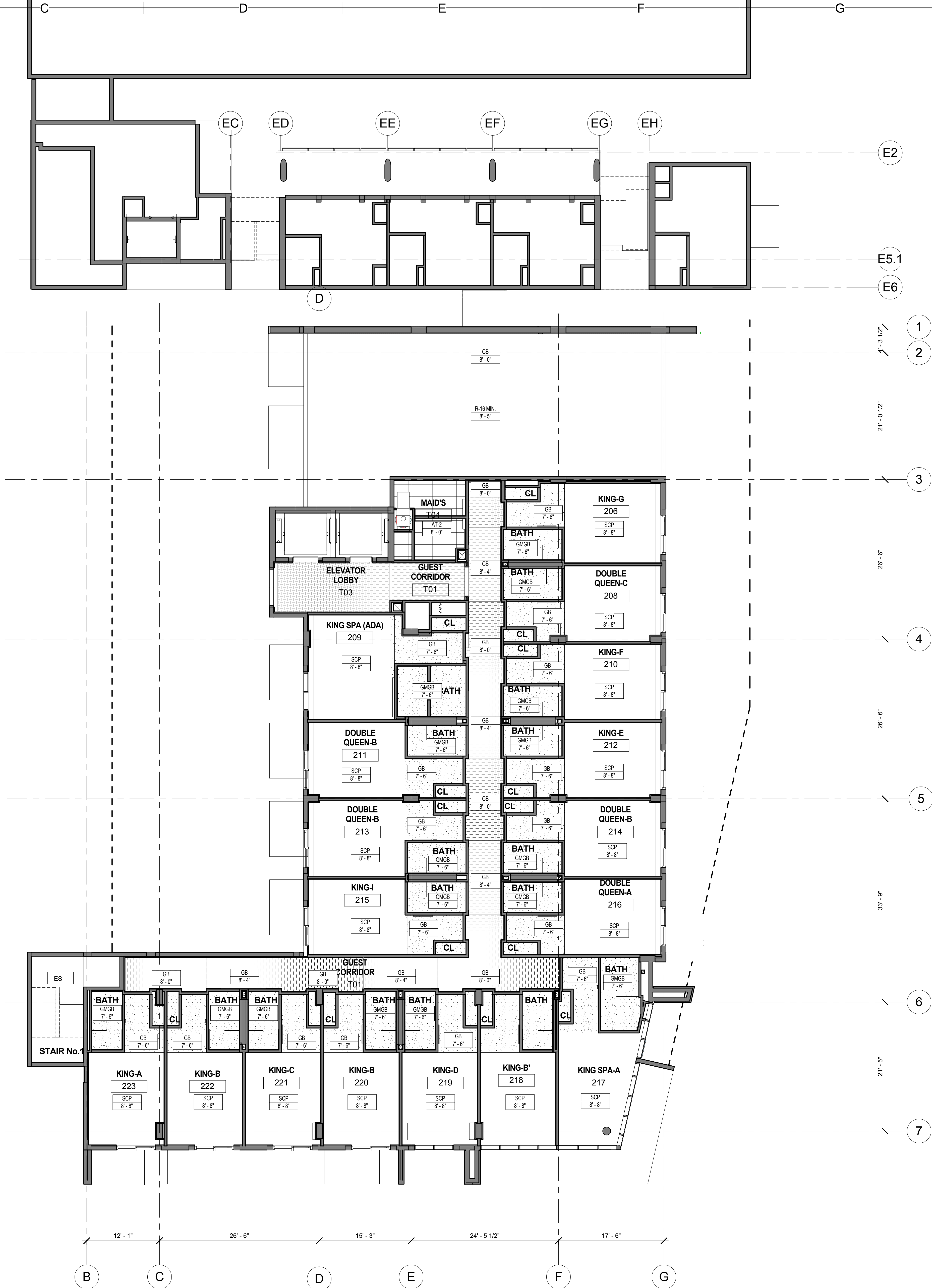
1 A6.02 LEVEL 200 REFLECTED CEILING PLAN 1/8" = 1'-0"
