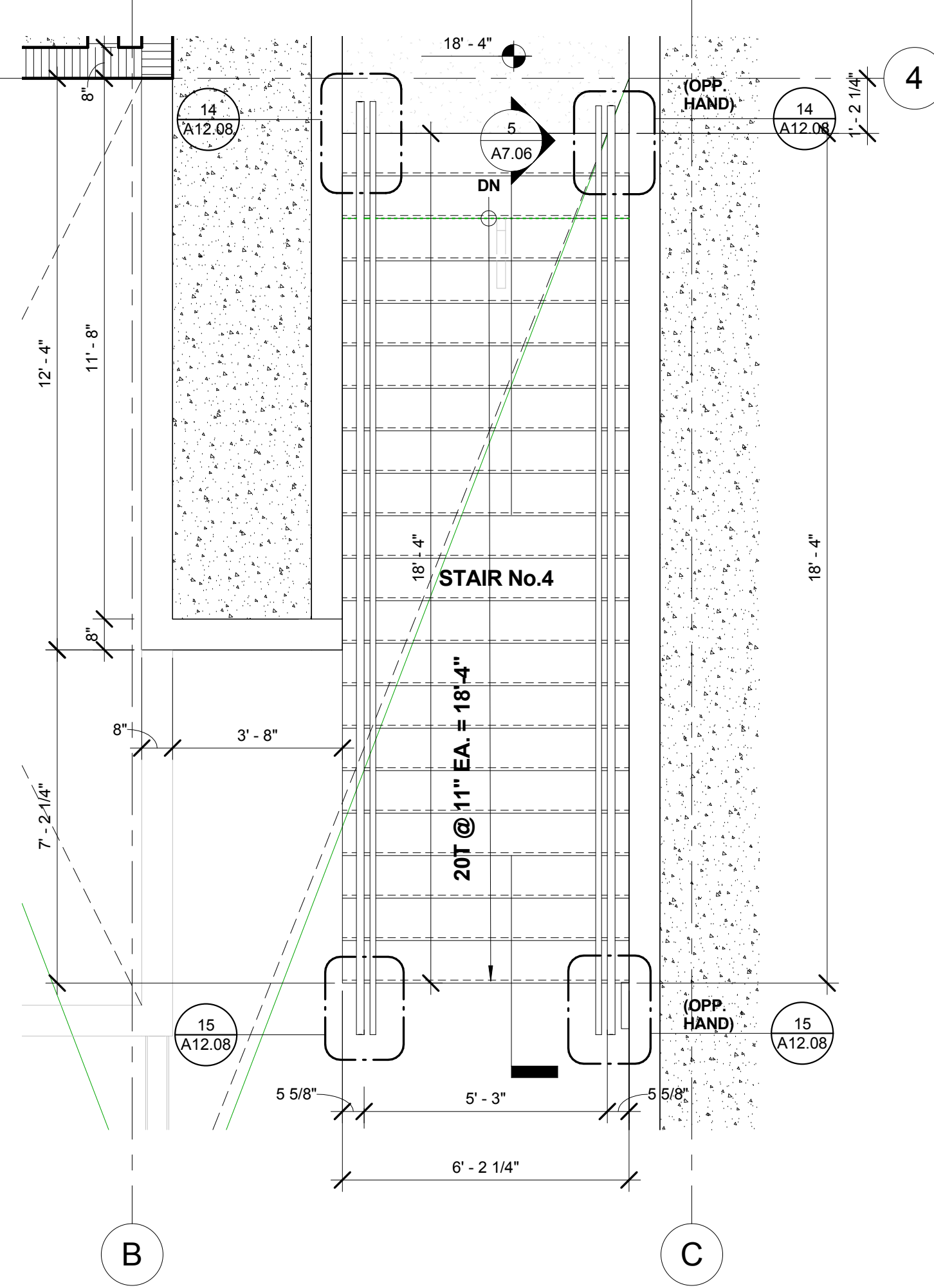
STAIR 04 - LEVEL 200
