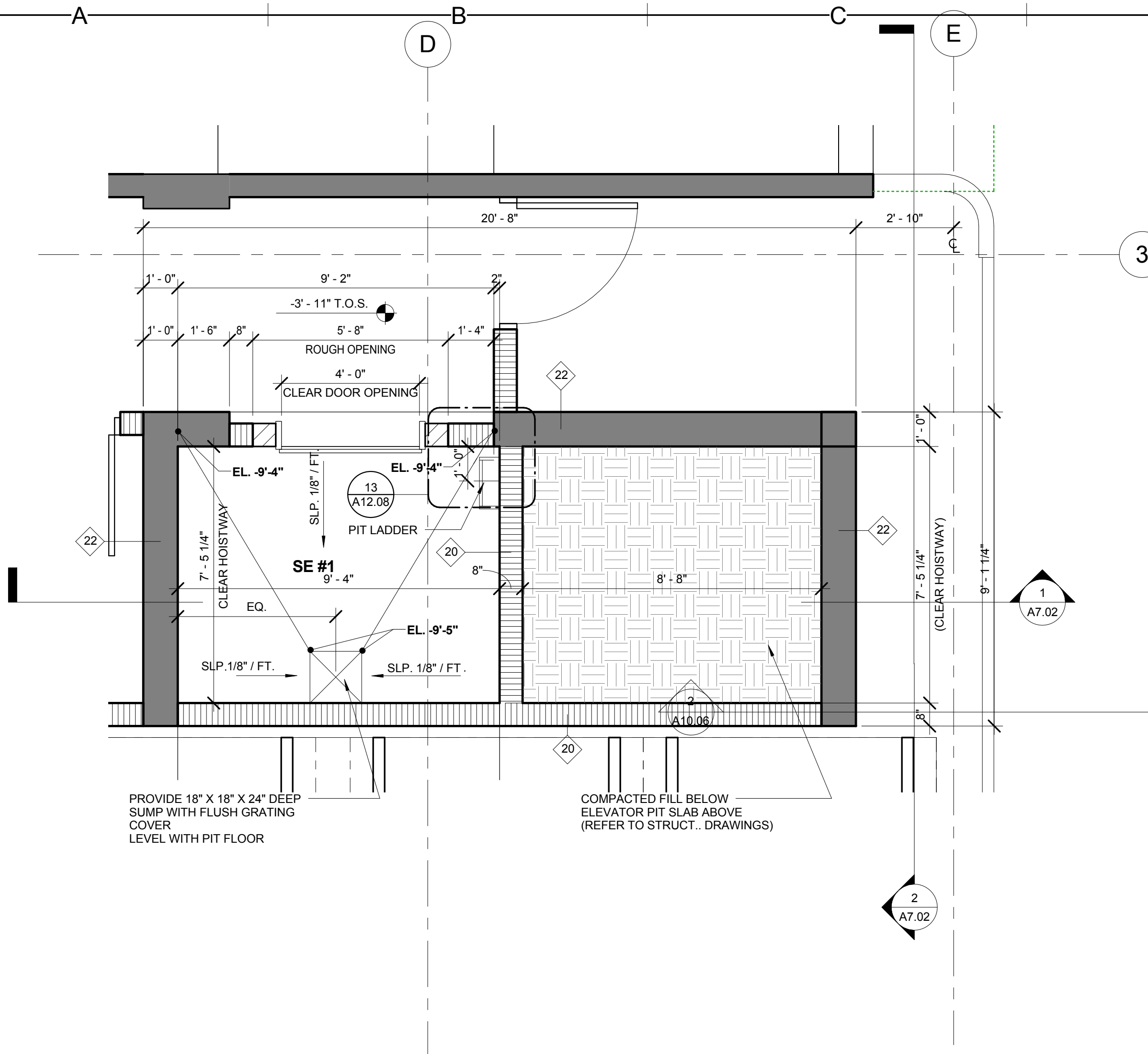
1 A7.00 ELEVATOR CORE - PIT PLAN 3/8" = 1'-0"
