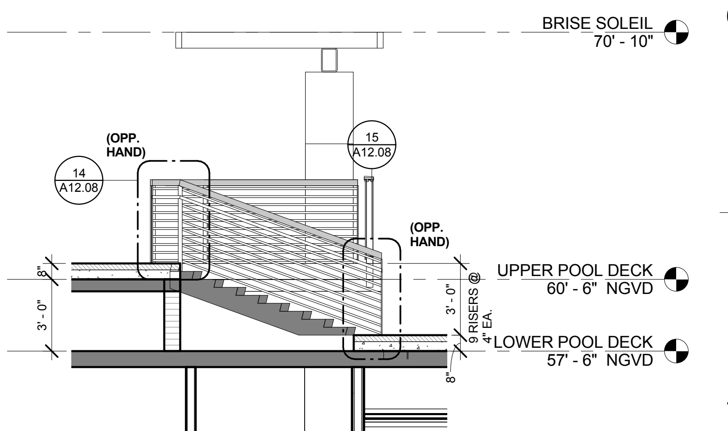
SECTION - STAIR 07
