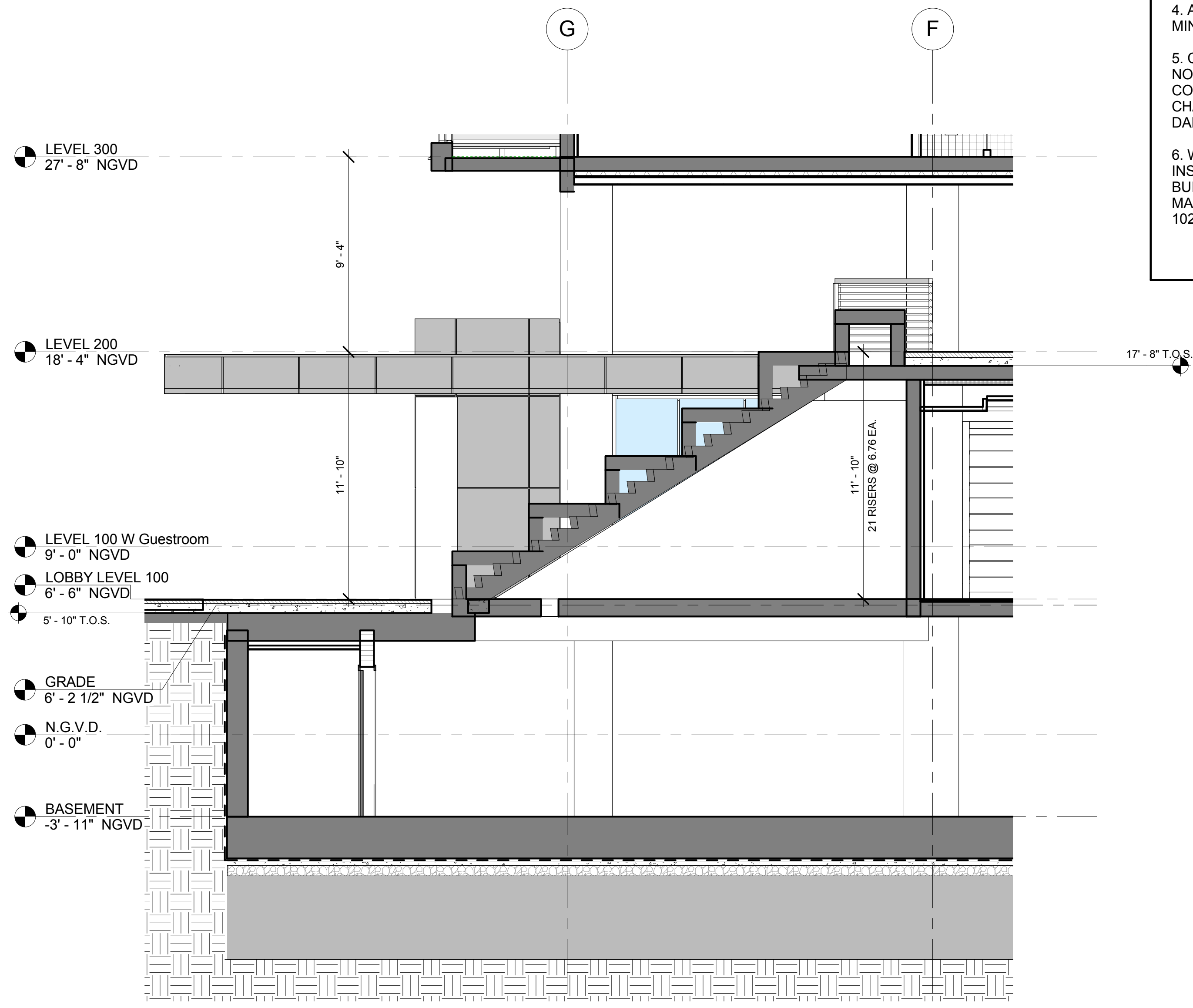
5 SECTION - STAIR 03 PEDESTAL STEPS
