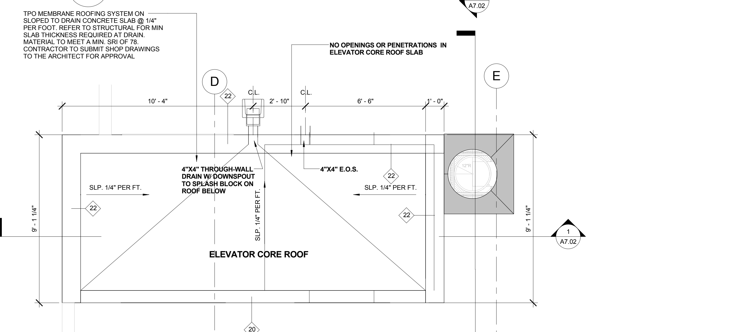
4 ELEVATOR CORE - OVERRIDE A7.01 3/8" = 1'-0"
